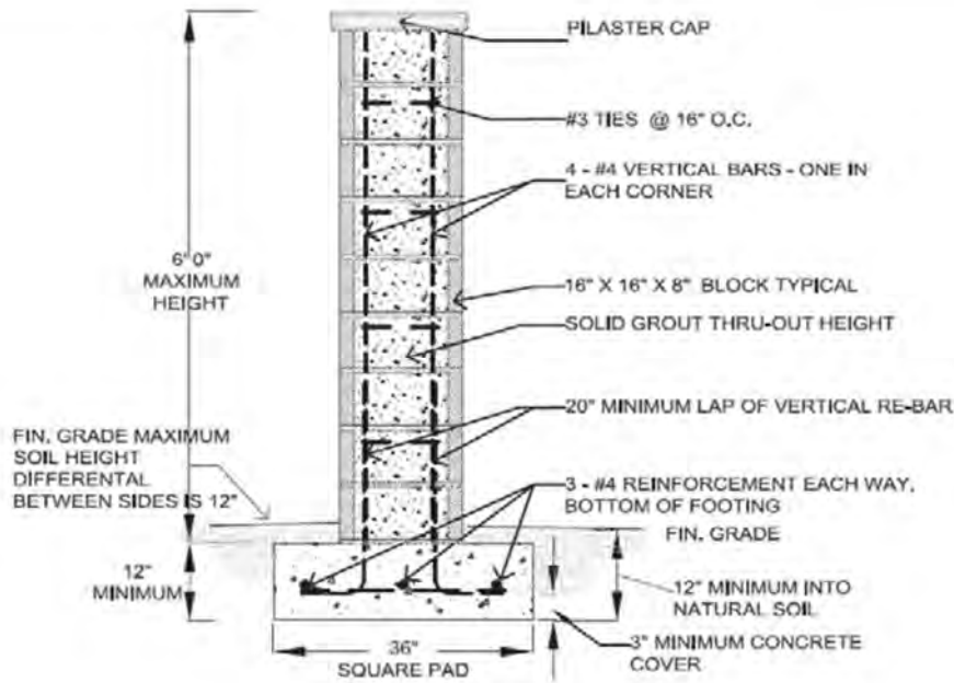
PILASTER SECTION
