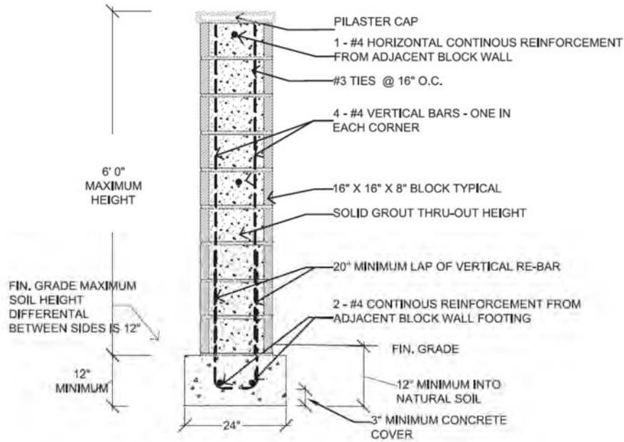
PILASTER SECTION
